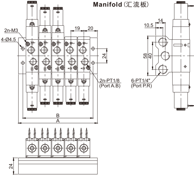
Manifold (汇流板)
